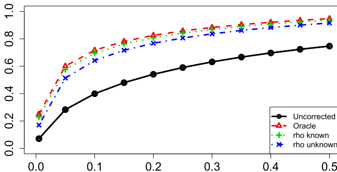
FIG. 1. X-axis: targeted FDR level \alpha \in \{0.005, 0.05, 0.1, 0.15, 0.2, 0.25, 0.3, 0.35, 0.4, 0.45, 0.5\} , Y-axis: TDP (power) averaged over 100 replications for four different procedures (see text in Section S-1.3). The model is the one-sided Gaussian one with equicorrelation \rho = 0.3 . The parameters used are n = 10^6 , \Delta = 2.5 , k/n = 0.1 .
